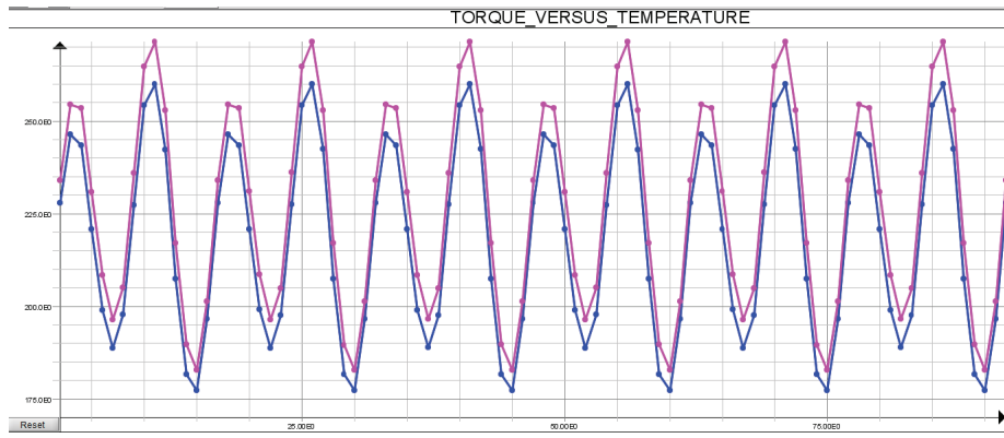
Figure 12: torque versus rotor position for 20°C and for 172.7°C
