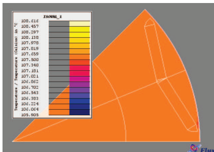
Figure 13: rotor temperature
