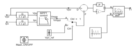
Fig. 4: Simple DC-DC converter control with MPP tracking.
