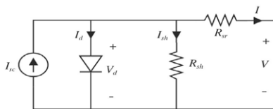
Fig. 1a: PV cell equivalent circuit.
