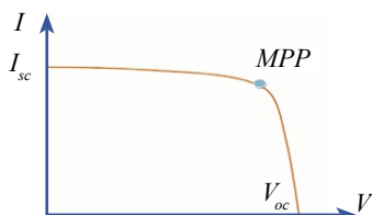
Fig. 1b: PV cell typical I-V characteristics.
