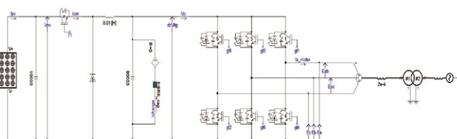
Fig. 2: Example of simulating a grid connected PV system simulation.
