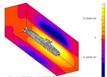
Scorpene SSK submarine and part of its load modelled with Flux (Courtesy of DCN).
