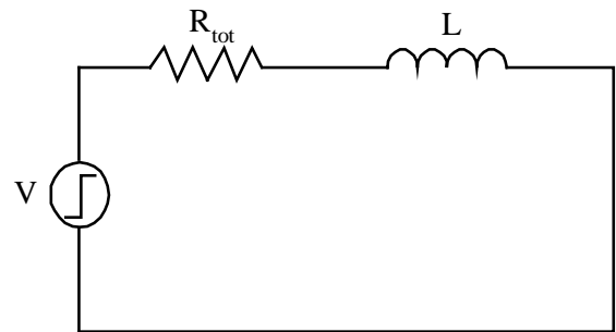
Fig 7: Machine one-phase representation with the rotor locked.
