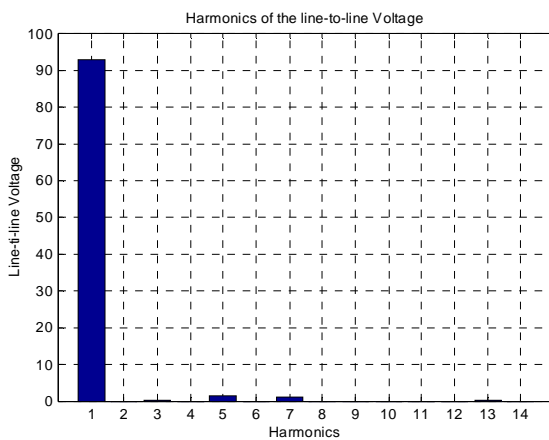
Fig 6: Line-to-line Voltage harmonic spectrum at 2000 [rpm].
