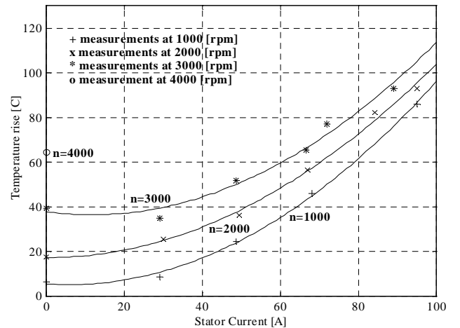
Fig. 10: Temperature rise at different speeds and different current loads.
