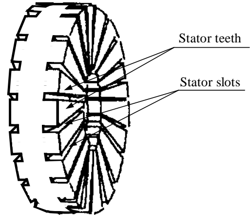
Fig 1: Torus machine with slotted stator.
