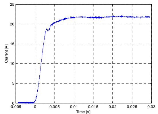
Fig 8: Current variation at the switching of the voltage supply.
