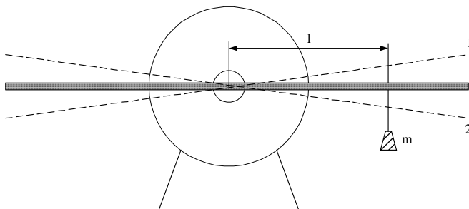
Fig. 9: Set-up for the measurement of the cogging torque [8].
