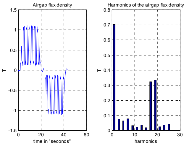
Fig 4: Airgap flux density at a radius R= 105 [mm] with Flux-3D for a non-salient pole machine at no-load.
