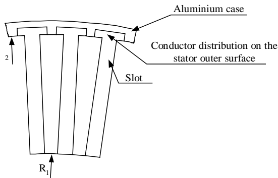
Fig. 3: Stator front section showing the conductors' distribution over the stator back.
