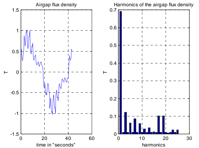
Fig 5: Airgap flux density at a radius R= 105 [mm] with Flux-3D for a non-salient pole machine at rated load.
